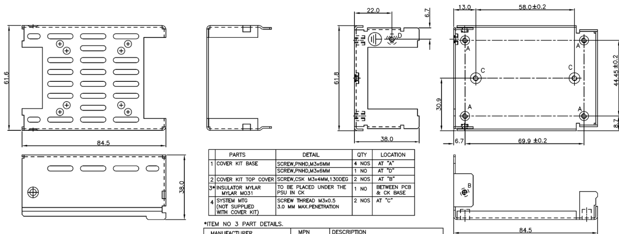
WLP120 and WLP75CK MECHANICAL OUTLINE DIMENSIONS
