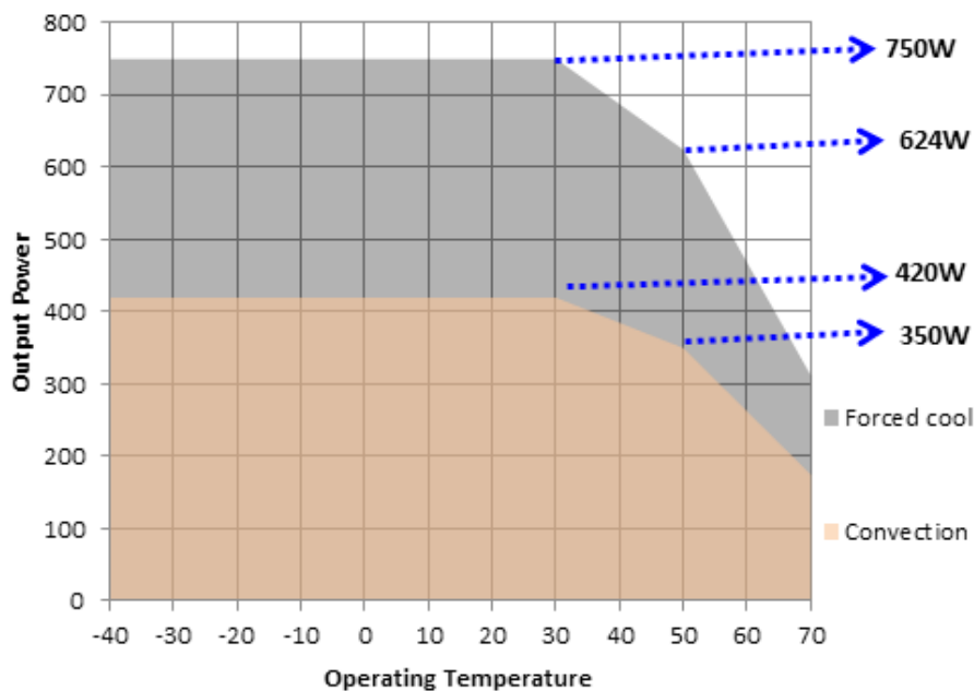
Derating Curve 24 V & above for slotted cover
